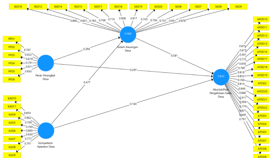
Figure 3: PLS Loading Factor (Bootstrapping)
