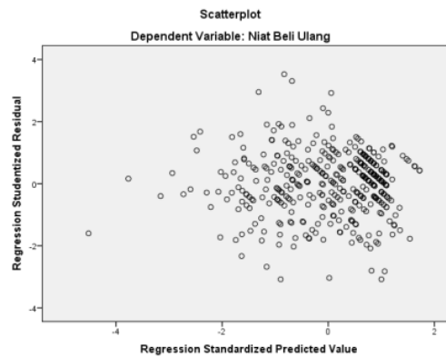
Figure 2: output of heteroscedasticity test results
