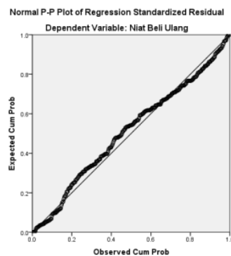
Figure 1: test result output (P-Plot)
