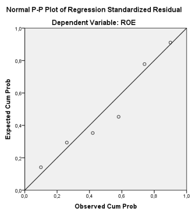
Gambar 1: Normal Profitability Plot
